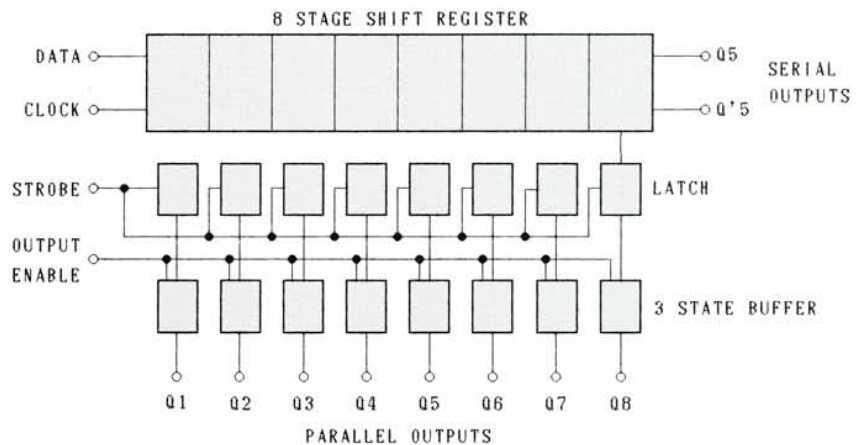
BLOCK DIAGRAM
