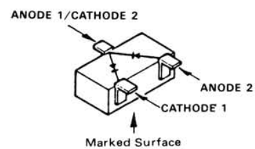
ISS226(C3) (D2001, 2004, 2008, 2009)
