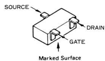
2SK302GR(TG)(Q1002, 1003)
