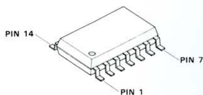
NJM2902M (Q2005, 2007, 2008, 2011)
