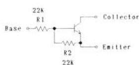
DTC124EK CIRCUIT DIAGRAM
