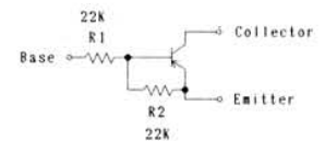
DTA124EK CIRCUIT DIAGRAM
