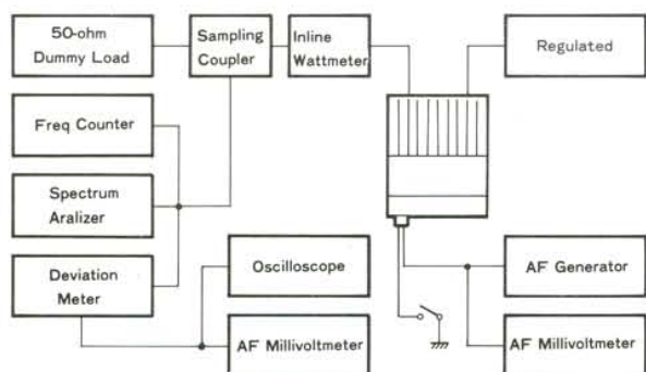
PLL & Transmitter Alignment Setup
