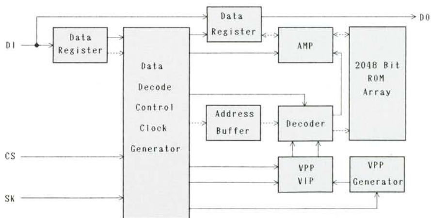
BLOCK DIAGRAM
