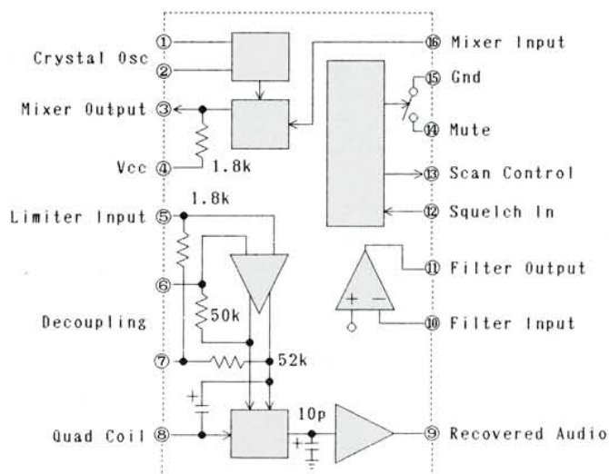
BLOCK DIAGRAM
