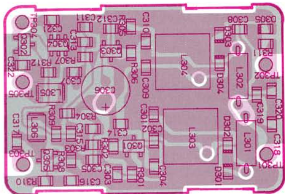
Obverse View of "Mixed Component" Side
