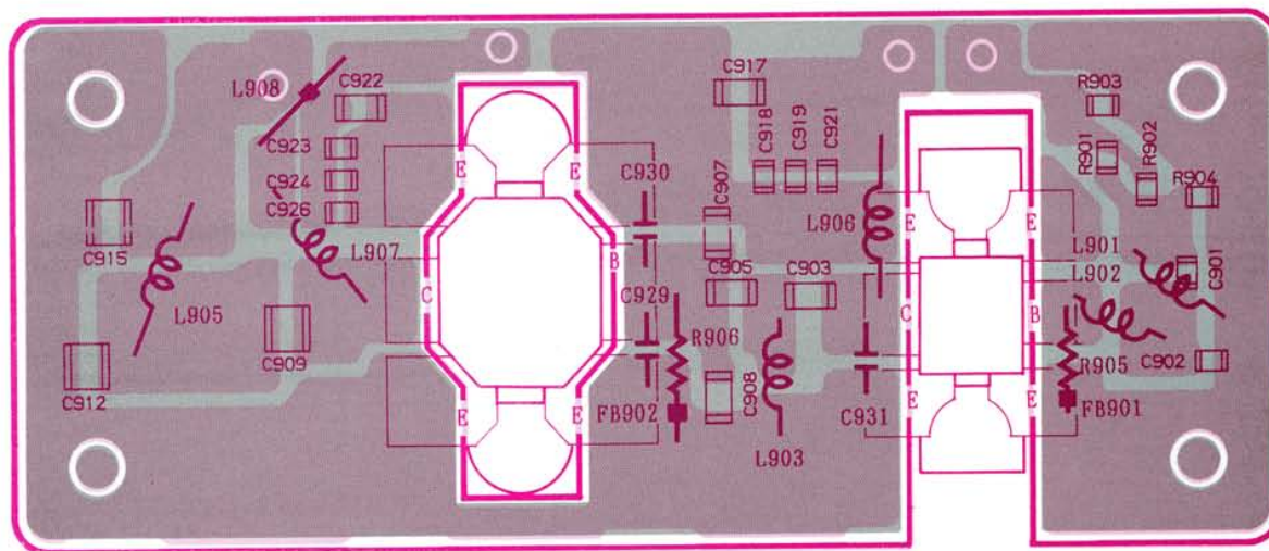
Obverse View of "Mixed Component" Side
