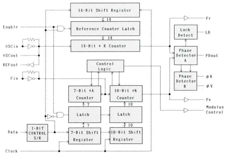
BLOCK DIAGRAM
