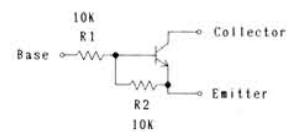
DTC114EK CIRCUIT DIAGRAM
