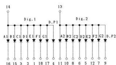
GL7S201J CIRCUIT DIAGRAM
