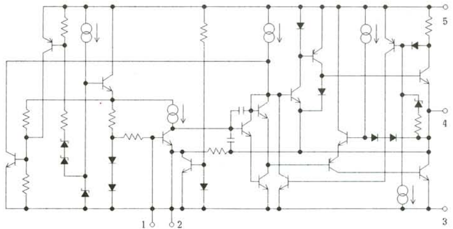
SCHEMATIC DIAGRAM
