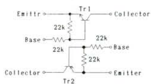
IMD2 CIRCUIT DIAGRAM
