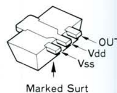
RH5VA32AA(D5)(Q2021)
