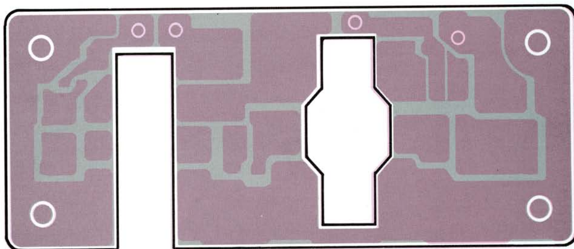
Obverse View of Solder Side
