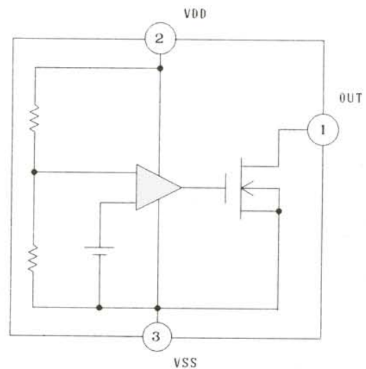
BLOCK DIAGRAM
