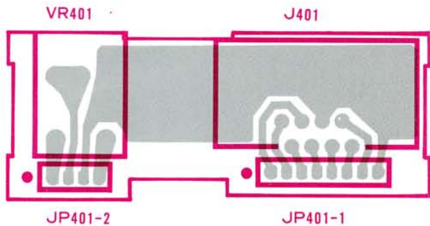
Obverse View of Component Side
