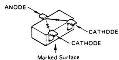
ISS181(A3) (D2002, 2007, 2010)
