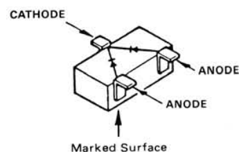
ISS184(B3) (D2003, 2006)
