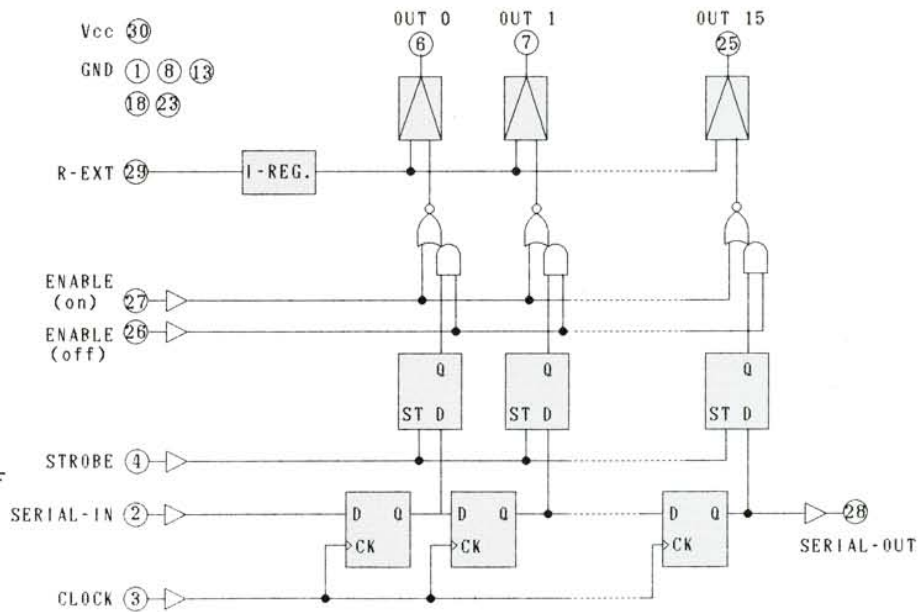
BLOCK DIAGRAM
