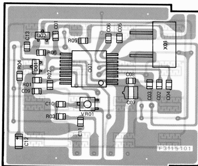
Obverse view of "chip-only" side
