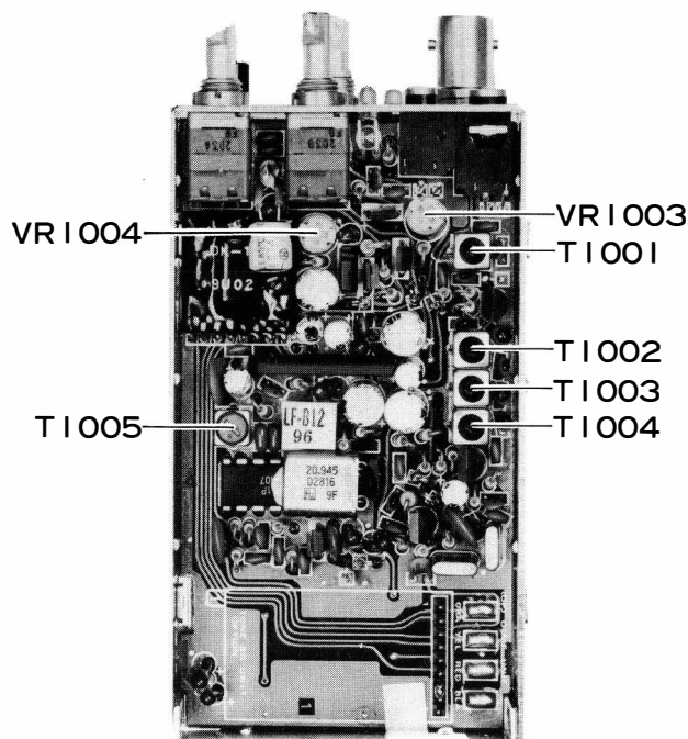
Receiver Alignment Setup
