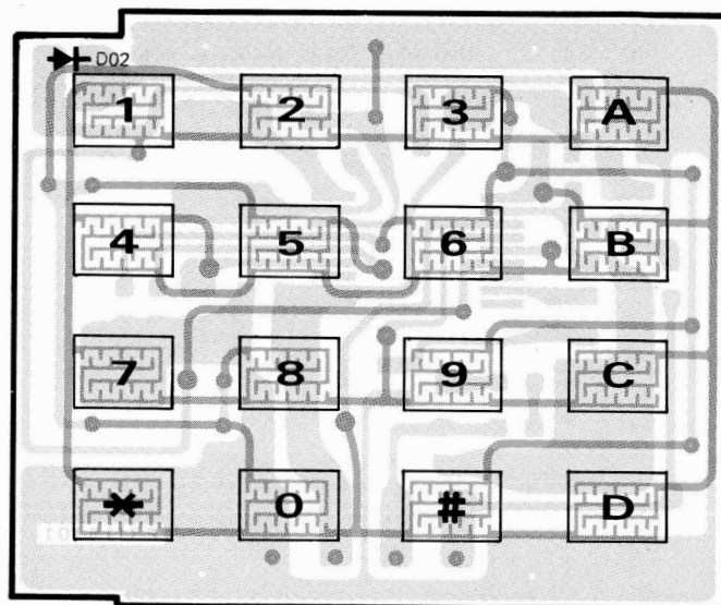
Obverse view of "Key mold" side
